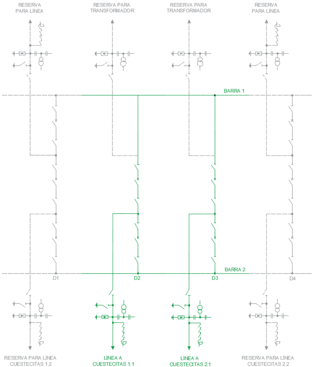
FIGURA 2. COLECTORA 500 kV
